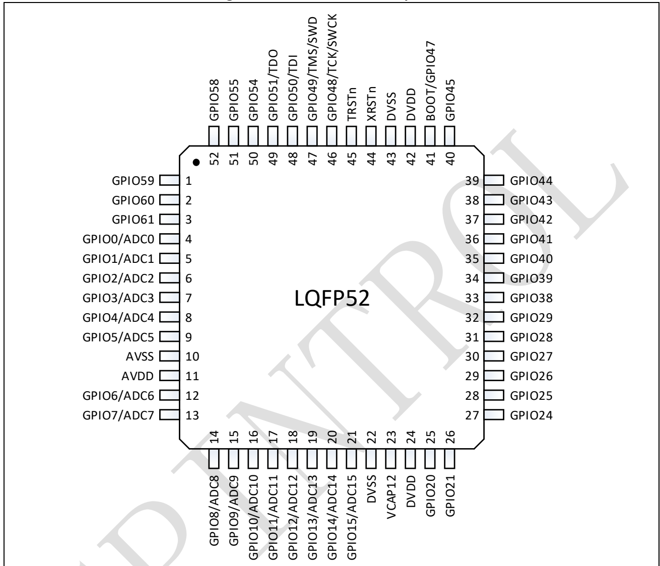
Figure 3-3: SPC1198 LQFP52 pinout
