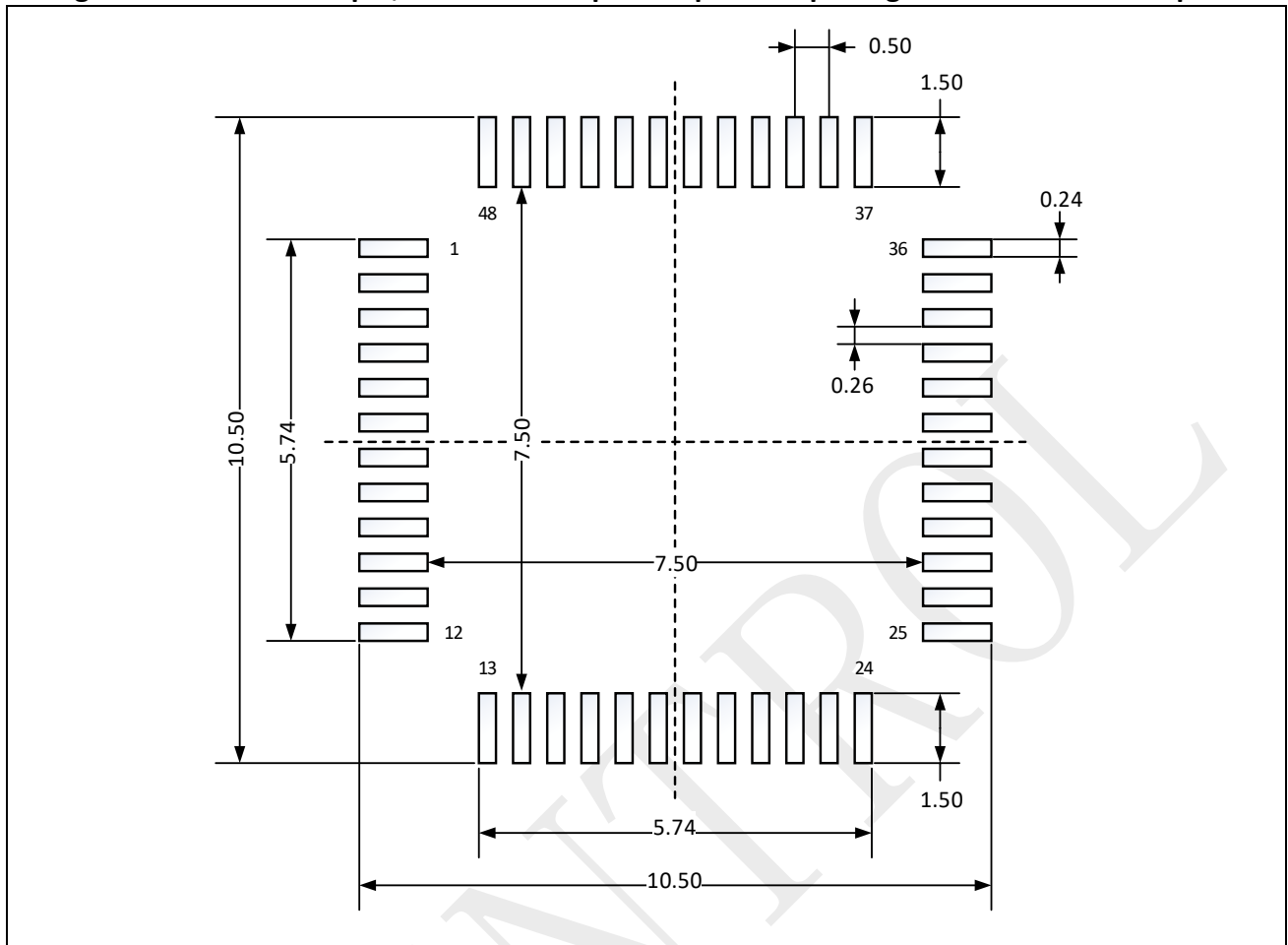
Figure 6-8: LQFP48–48 pin, 7 x 7 mm low-profile quad flat package recommended footprint
