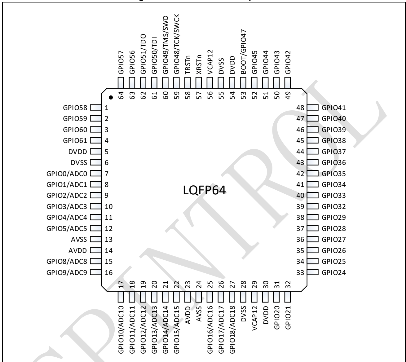
Figure 3-2: SPC1198 LQFP64 pinout
