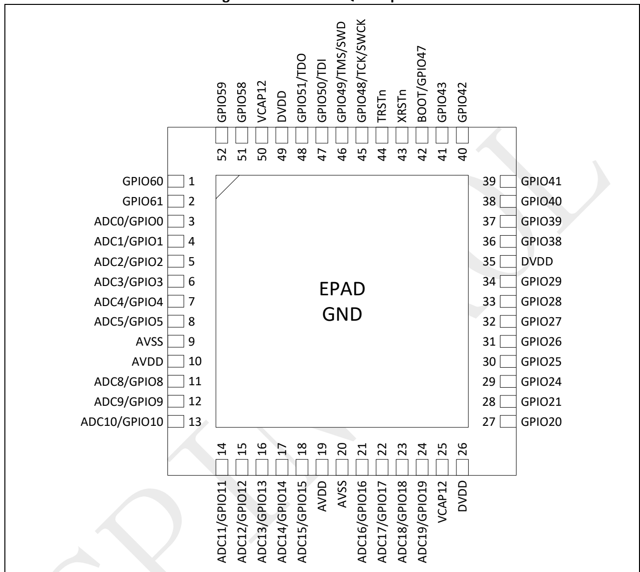
Figure 3-5: SPC1198 QFN52 pinout
