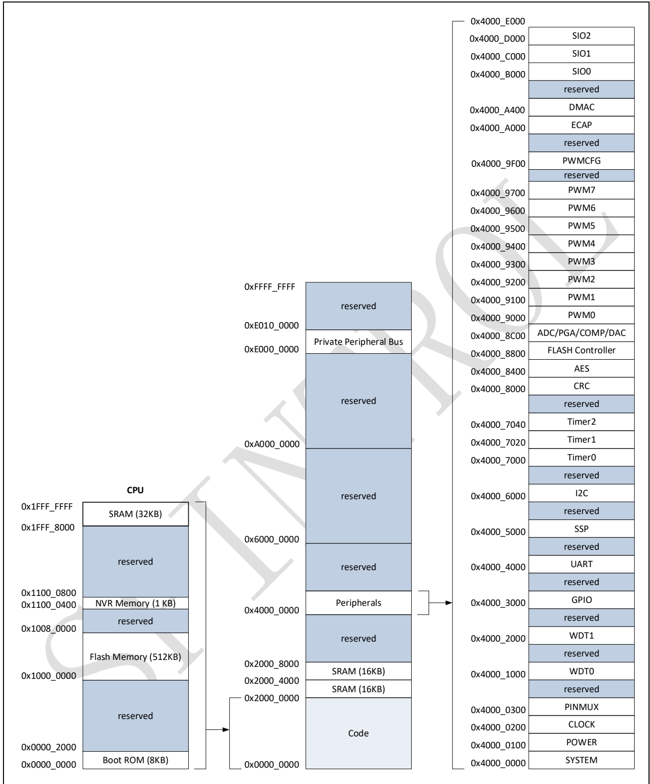
Figure 4-2: SPC1198 memory map with Cache enabled
