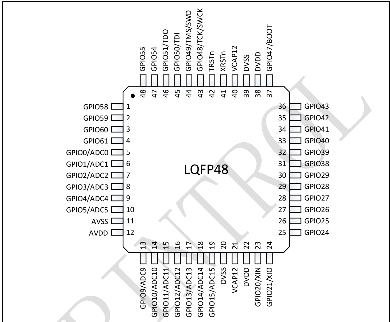
Figure 3-4: SPC1198 LQFP48 pinout
