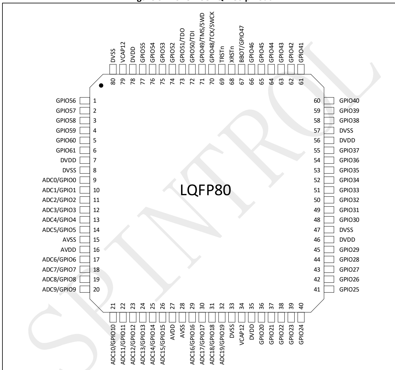
Figure 3-1: SPC1198 LQFP80 pinout
