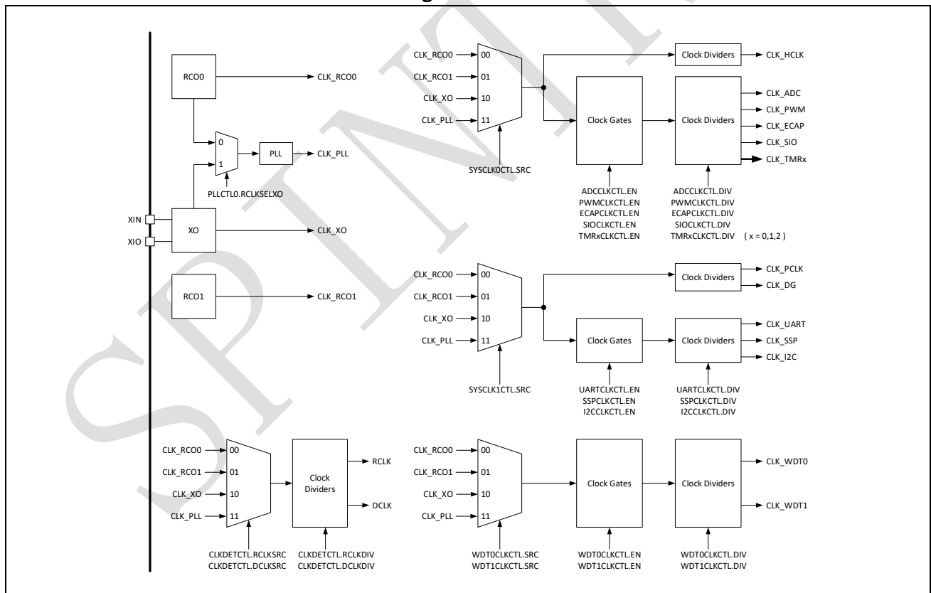
Figure 2-1: Clock tree
